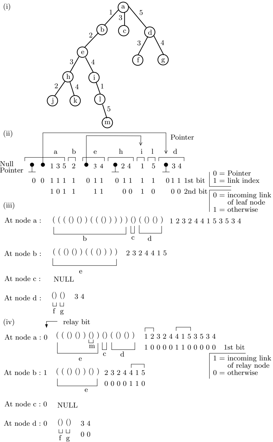
Fig. 3. (i) Multicast Tree (ii) Link+ encoding (iii) Link* encoding (iv) Link** encoding
