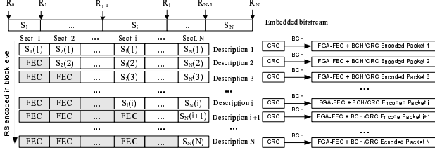
Fig. 2. Generalized FGA-FEC with product codes
