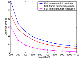
Fig. 3. D(R) curves at various adaptation levels.
